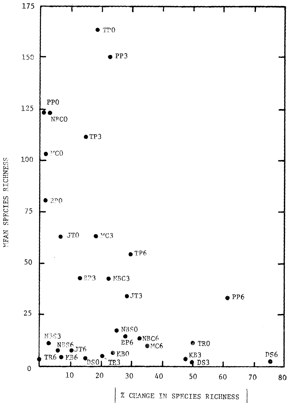
Figure 2. Intertidal species richness (mean of the first and second years) by study area - tide height compared with the percentage change in species richness between the first and second years. BP6 = Beckett Point +6', BP3 = Beckett Point +3', BPO = Beckett Point +0'; DS6, DS3, DS0 = Dungeness Spit +6', +3', +0'; JT6, JT3, JTO = Jamestown +6', +1.4', +0'; KB6, KB3, KB0 = Kydaka Beach +6', +3', +0'; MC6, MC3, MCO = Morse Creek +6', +3', +0'; NBC6, NBC3, NBC0 = North Beach Cobble +6', +3', +0'; NBS6, NBS3, NBS0 = North Beach Sand +6', +2', +0'; PP6, PP3, PPO = Pillar Point +6', +3', +0'; TP6, TP3, TPO = Tongue Point +6', +3', +0'; TR6, TR3, TR0 = Twin Rivers +6', +3', +0'.
